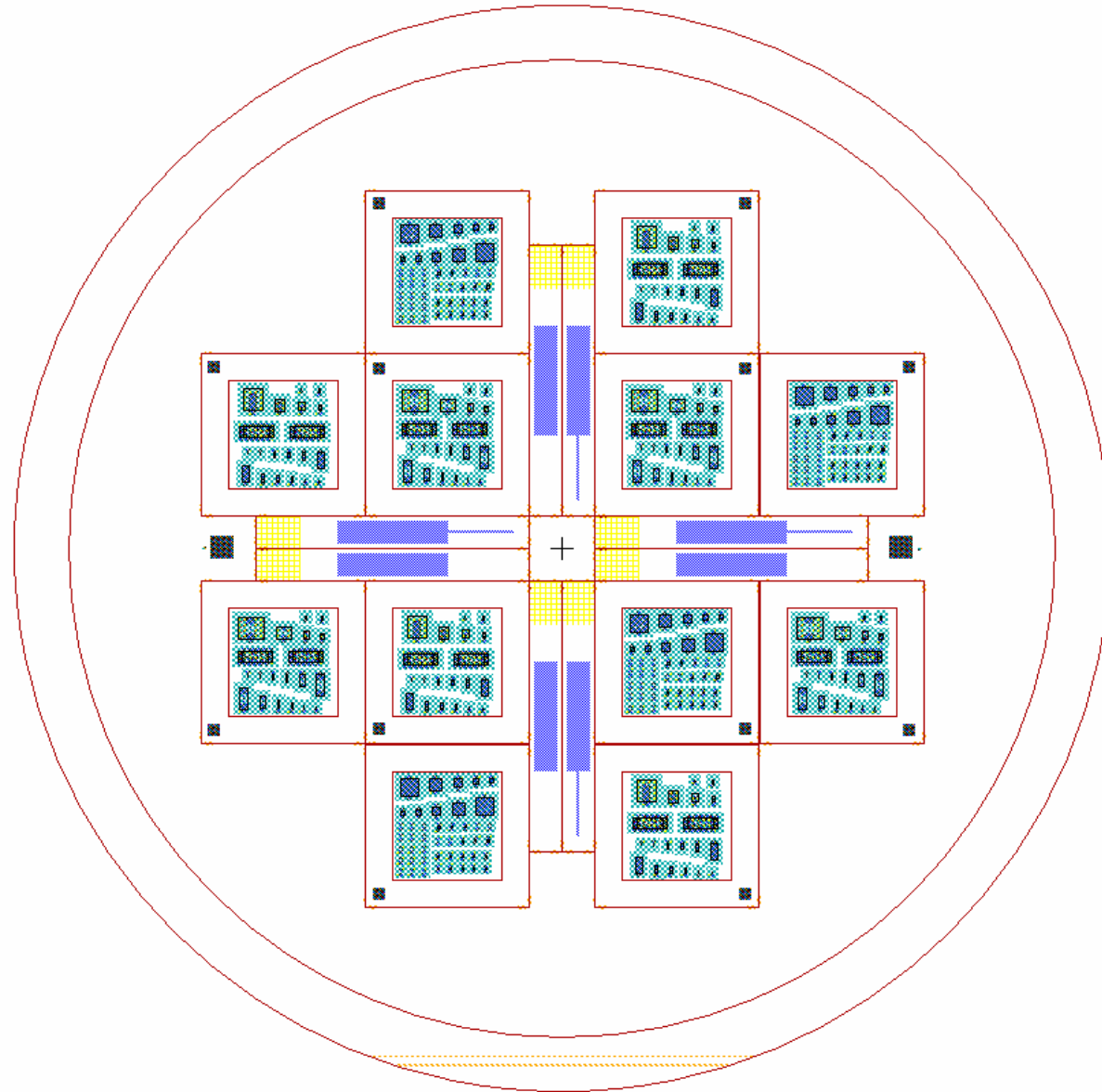
Design overview of the test wafer developed by the project. Twelve 15x15 mm squares contain a large number of basic design elements. Eight rectangles are dedicated to four-point bending tests to be performed after dicing of the wafer.
