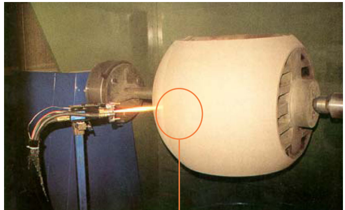
Oxidized and worn surfaces in erosion-corrosion
