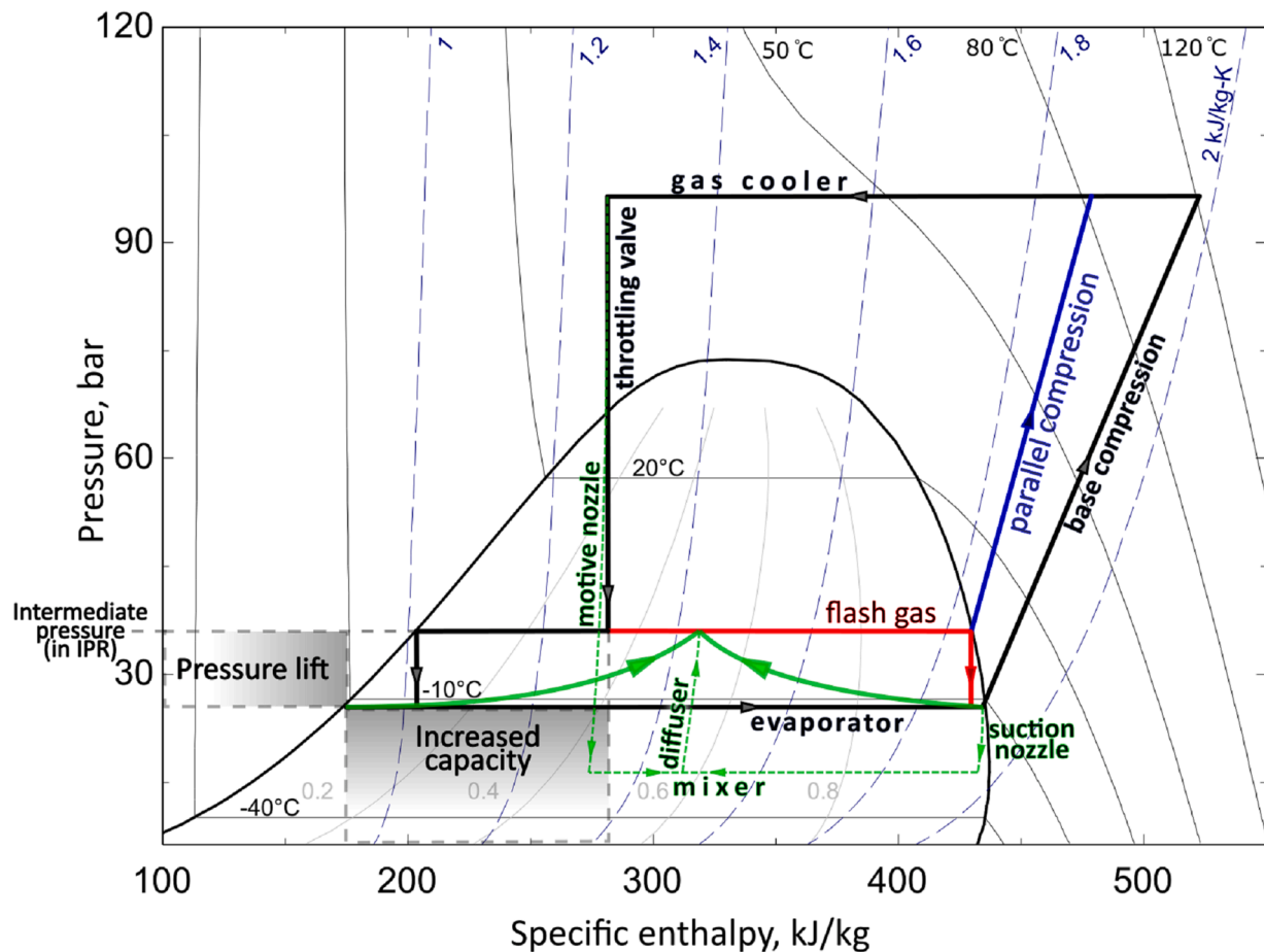
Fig. 5. P - h diagram of the R-744 booster system for RSW with PC, FGBV and ME. The processes for PC, flash gas bypass and ME are shown with blue, red and green colours, respectively, with the permission of Bodys et al. (2018). For the application shown in Fig. 3, there is no ME, hence the diagram must be without green lines. For the application shown in Fig. 4, there is no flash gas.
