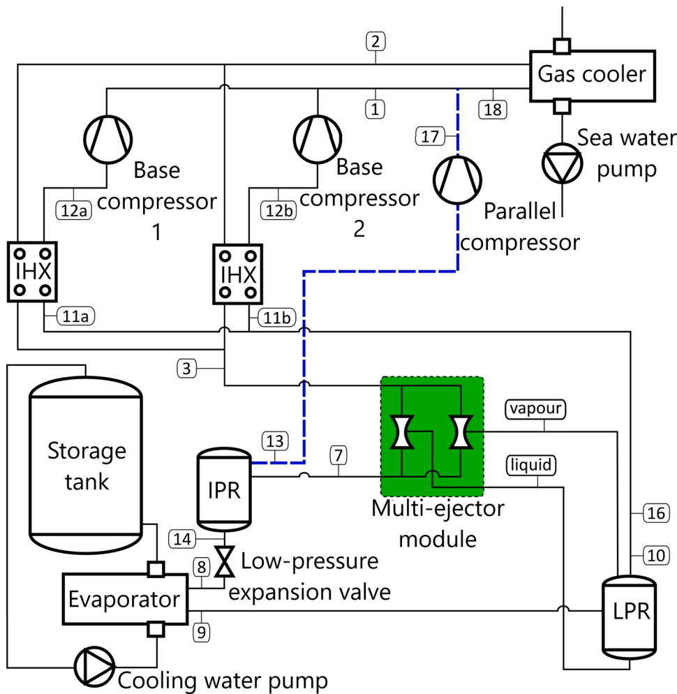
Fig. 4. . The layout of R-744 booster system for RSW with ME with the permission of Bodys et al. (2018). The flow direction is clockwise. 12a-1 and 12b-1: base compression, 1–2: heat removal through the gas cooler, 3–7: throttling and mixing in the multi-ejector, 8–9: evaporation, 9–10: vapour refrigerant from the evaporator to low-pressure receiver, 10–11a and 10–11b: vapour refrigerant from low pressure receiver to the base compressors, 14–8: expansion to the evaporator by expansion valve, 13–17: compression of intermediate-pressure vapour refrigerant to high-pressure by the parallel compressor.
