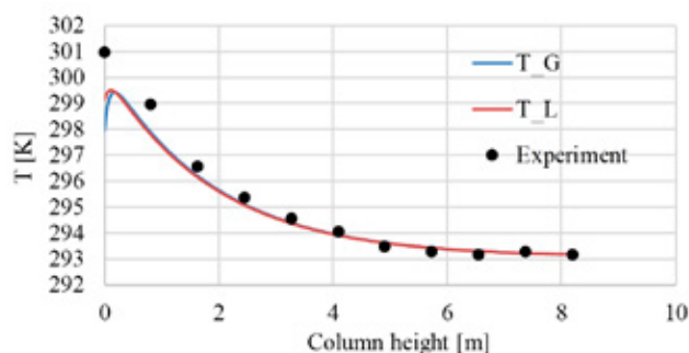
Model validation
