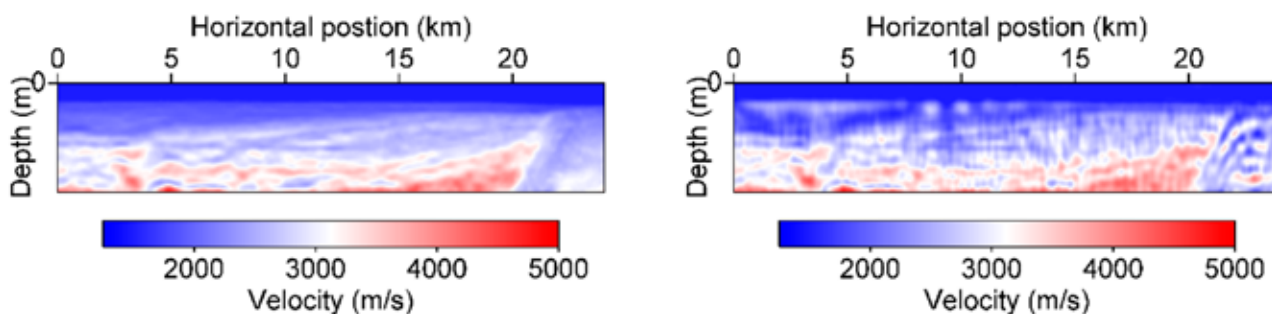
Figure 1: Selected results from Task 12 in 2018. [left] P-wave interval velocity model in depth for a subset of the Inline 1024 from Gassnova's seismic cube GN1101. [right] P-wave velocity model derived from FWI for the subset of Inline 1024 (from Dupuy et al. 2018, to be published).
