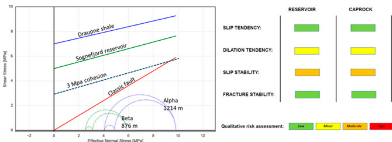
Figure illustrating 2018's main results from fault slip stability screening illustrating the need to better constrain the fault strength properties (cohesion) for Smeaheia in order to reduce the risk related to fault reactivation. Qualitative risk level shown for different methods addressed.
