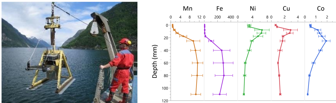
Figure 6: Vertical profiles of metals in pore water measured with DGT-probes in box core sediment samples from an abandoned sea deposit for ilmenite tailings. The profiles show near-surface mobilisation of nickel, copper and cobalt, but no upwards diffusion of nickel, copper and cobalt from deep deposit layers. The depth scale on the profiles indicates depth in sediment.
