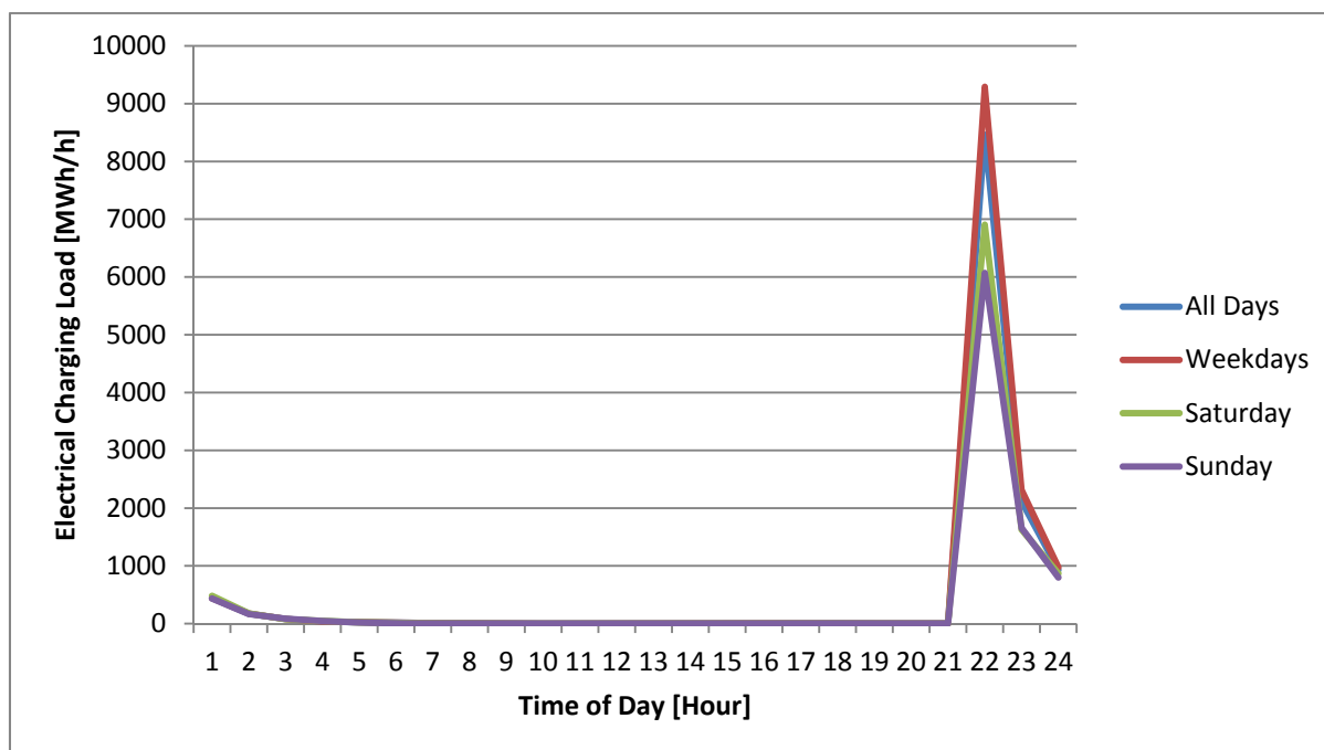
Figure 3-9 Electrical Load of 11.04kW Timed Charging in Denmark
