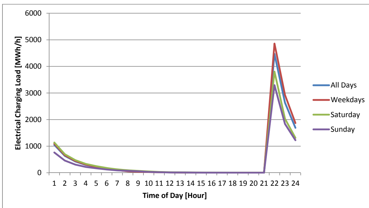
Figure 3-8 Electrical Load of 3.68kW Timed Charging in Denmark
