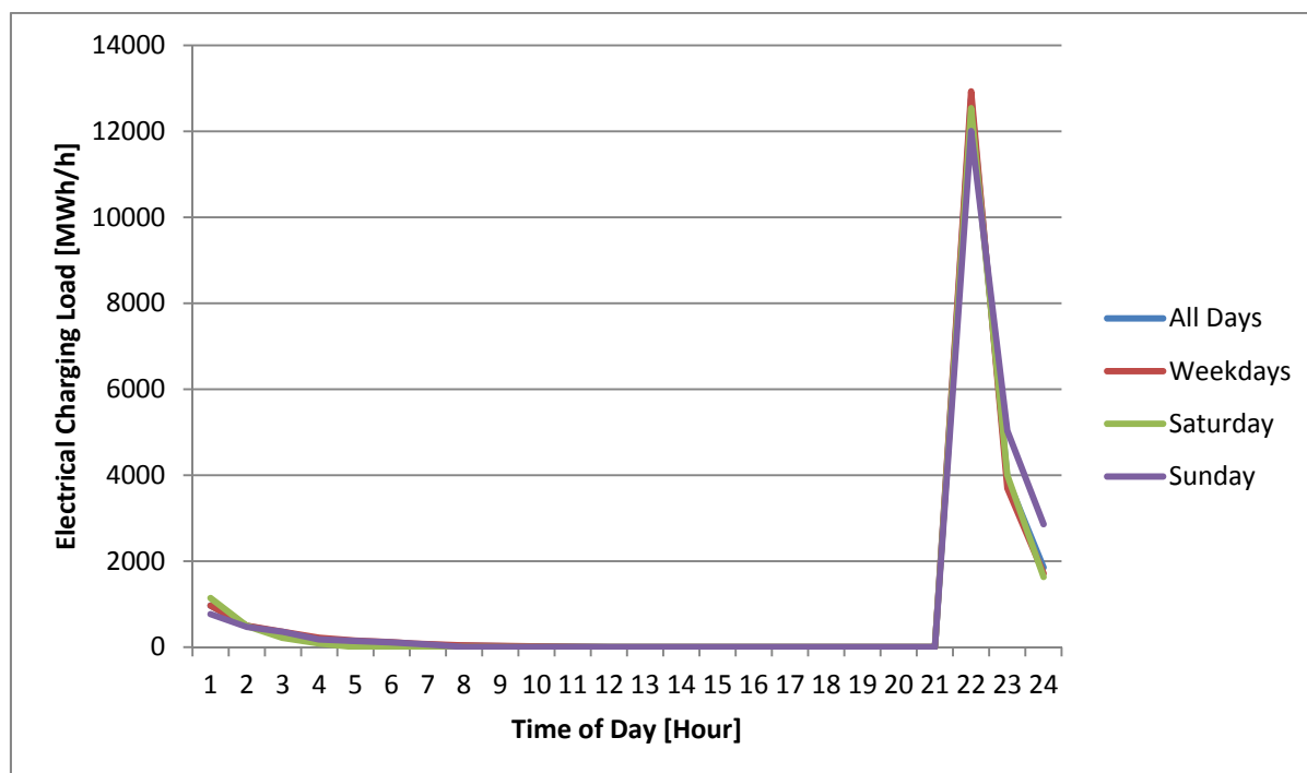
Figure 3-57 Electrical Load of 11.04kW Timed Charging in Finland
