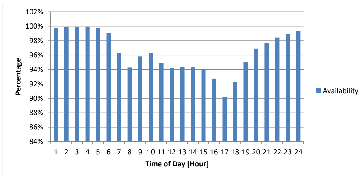
Figure 2-10 Overall EV Hour Availability Data (All-Day) in Sweden
