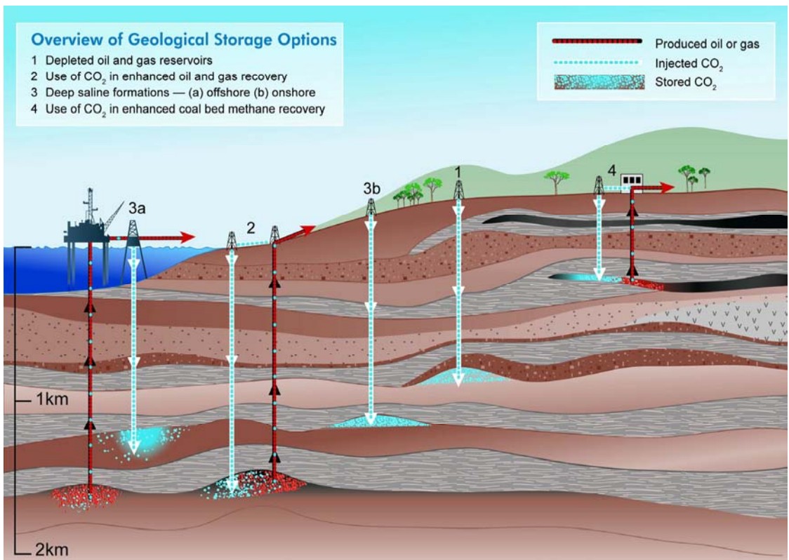
Figure 3.7. Underground storage alternatives (IPCC 2005).
