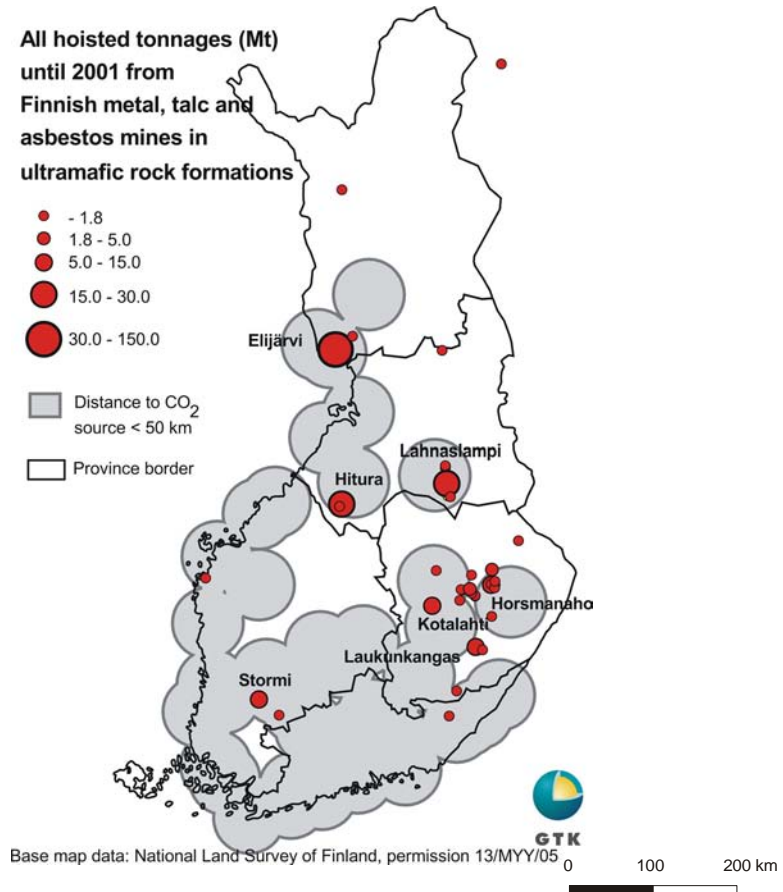
Figure 4.9. Possible sources of serpentinite in Finland. Circles mark areas where the distance to a major stationary CO 2 emitter is < 50 km (Aatos et al. , 2006; Teir et al. , 2006).
