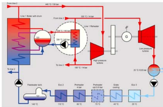
Reheating-scheme. (© City of Amsterdam Waste and Energy Company)
