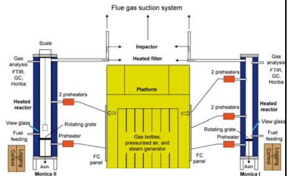
The two multi-fuel reactors at SINTEF
