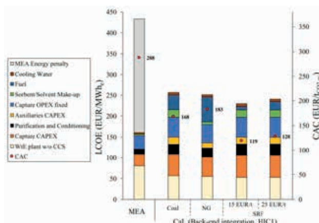
LCOE and CAC for the WtE plant with CO 2 Capture.
