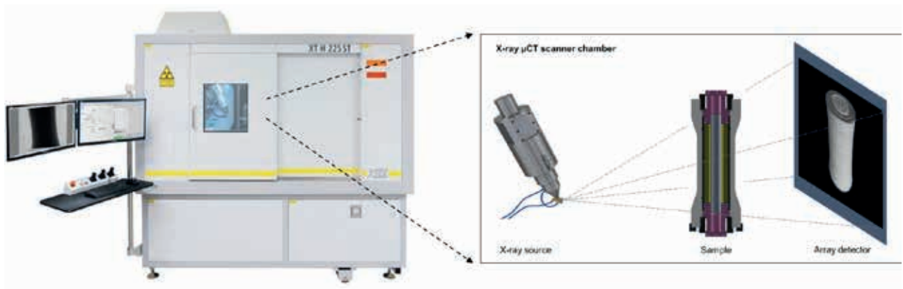
The ECCSEL well integrity research infrastructure. This mini-wellbore simulator is used for in-situ investigation of cement integrity under CT imaging. Sketch by A. Ghaderi.
