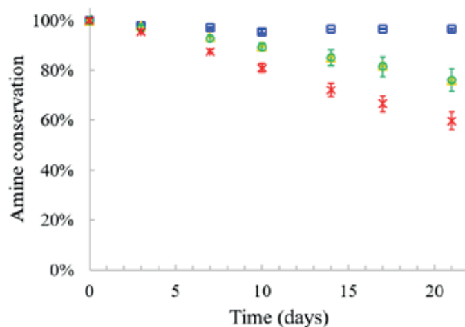
Amine conservation (%) as a function of time (days) for oxidative degradation experiments without (red markers - basecase) and with various salts added (yellow, green, blue).
