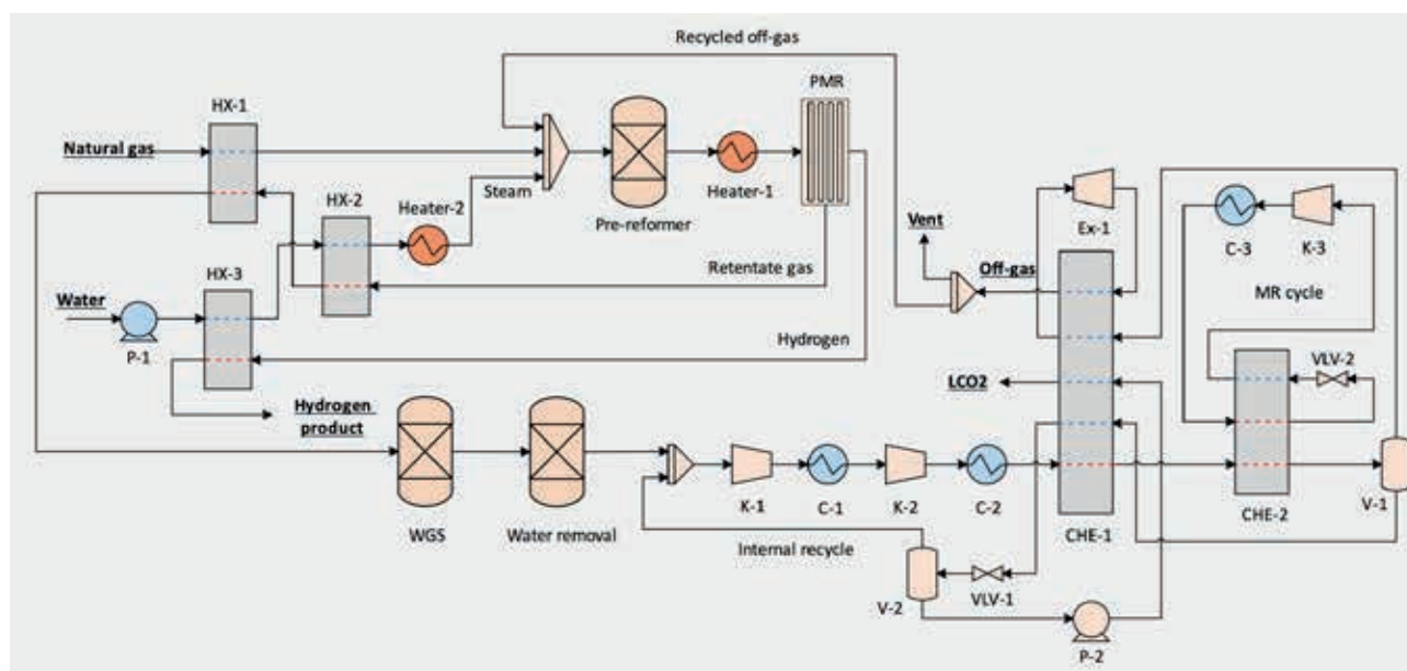
Detailed process flow diagram of hybrid PMR and CO 2 -liquefaction process with off-gas recycle and WGS reactor after PMR.
