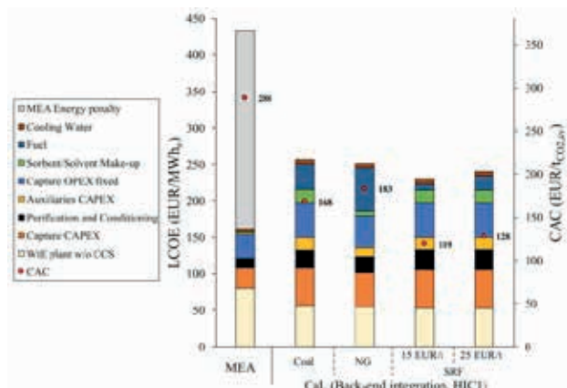
LCOE and CAC for the WtE plant with CO 2 Capture 9
