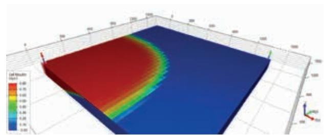
CO 2 injection with mobility control
