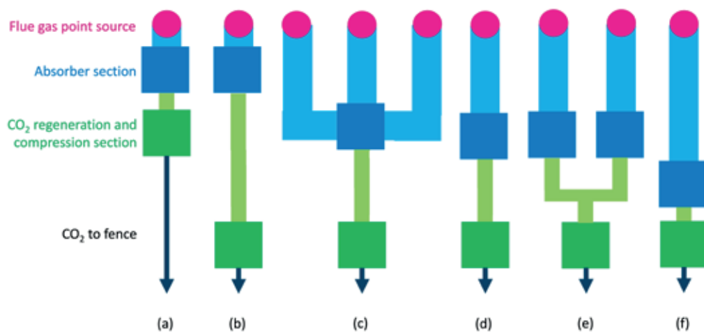
Illustration of different layout alternatives that could be considered in the case of an industrial cluster.
