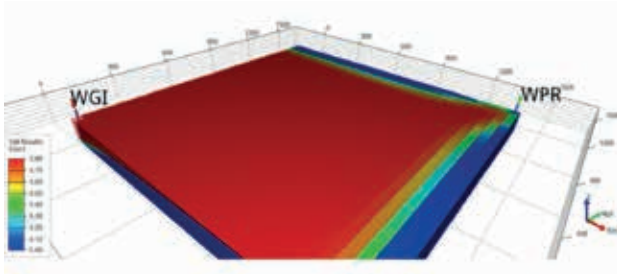
CO 2 injection without mobility control
