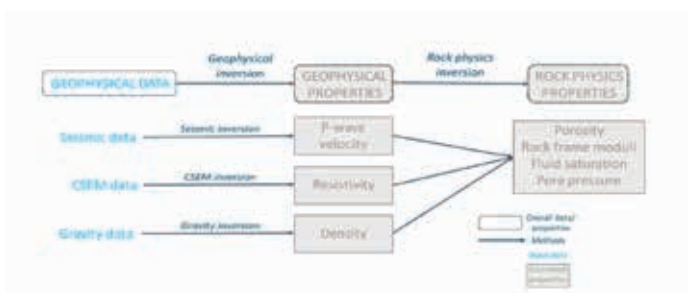
Two-step workflow combining geophysical and rock physics inversion.
