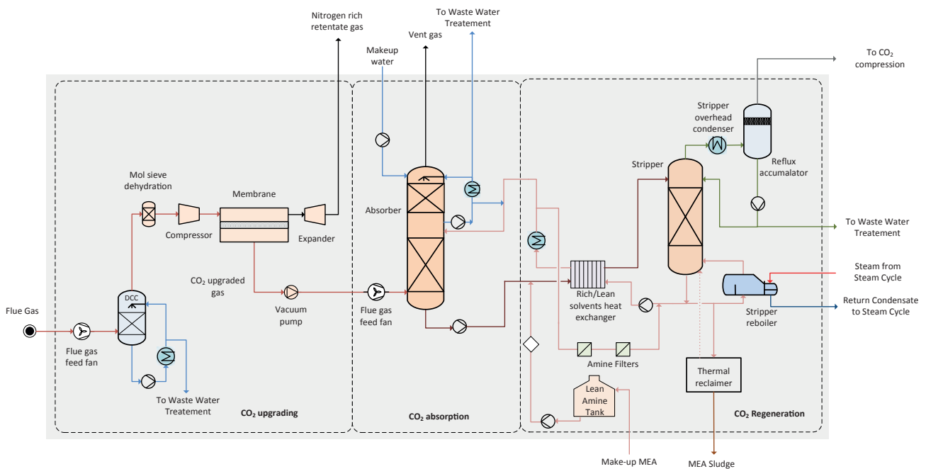
Membrane-absorption hybrid system layout.
