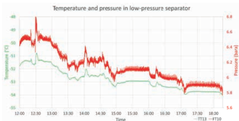
Pressure and temperature in the final separation stage for liquefaction of pure CO 2
