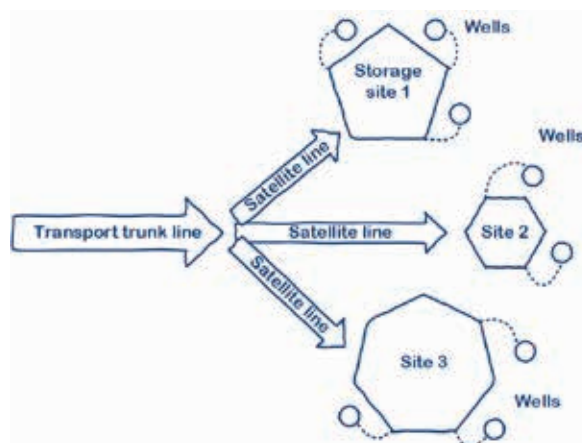
Generic illustration of a transport and storage network for a CO 2 storage hub with several sites.
