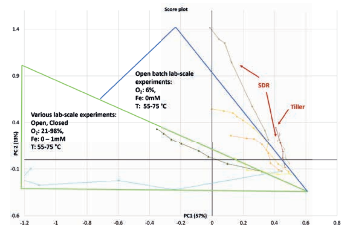
Score plot from Principal Component Analysis (statistical method to investigate dataset) over different lab experiments (batch and solvent degradation rig- SDR) and Tiller pilot (x-axes-Principal Component 1, y-axes-Principal Component 2). The figure shows that the open batch lab-scale experiments at low O 2 , in regard to degradation compounds profile, shows highest resemblance to cycled experiment (SDR) and pilot demonstration (Tiller).
