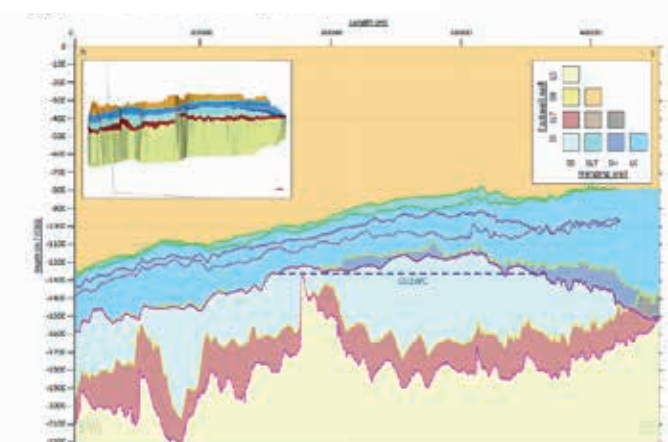
Vette Fault Zone Lithologic Juxtaposition
