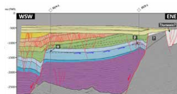
Seismic section with fault interpretation for Smeaheia (ref. Mulrooney et al, in prep).
