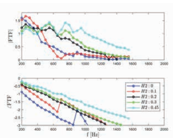
Flame Transfer Function -FTF- gain (top) and phase lag (bottom) for different hydrogen content.
