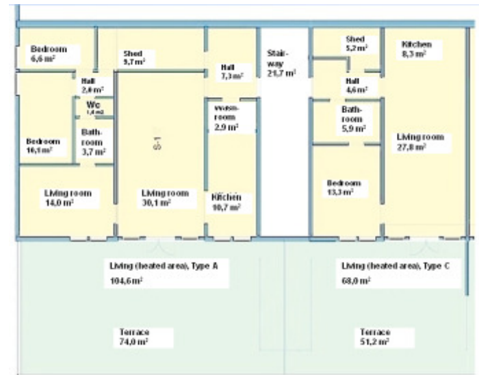
Plan of a large and a small ground floor apartment
