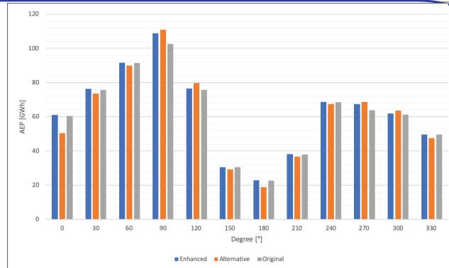
Figure AEP for different wind directions Table : Economic and environmental results for different layouts.
