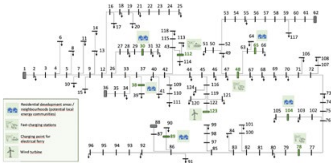
Figure 2 The CINELDI MV Reference grid – Flexibility case.
