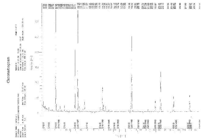
GC FID chromatogram of fatty acids from a single female C. finmarchicus
