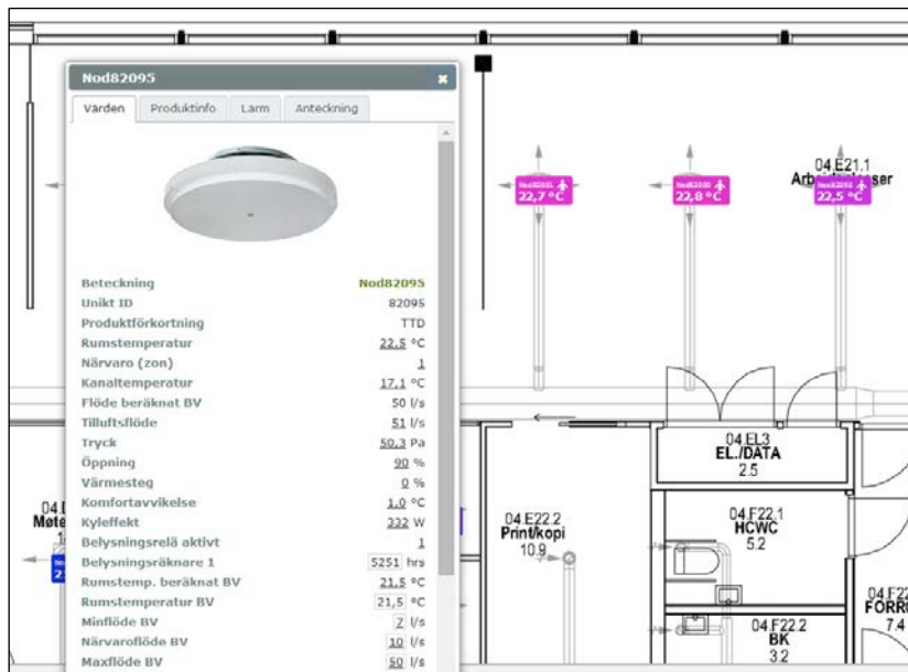
Figure 2: Remote control and monitoring of the supply airflow rate, supply temperature and room temperature for each diffuser of the building.
