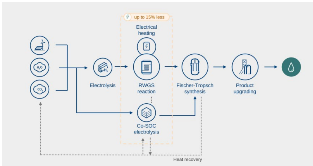
Figure 6-1 Flowchart of Norsk e-Fuel's planned process (Source: norsk-e-fuel.com)
