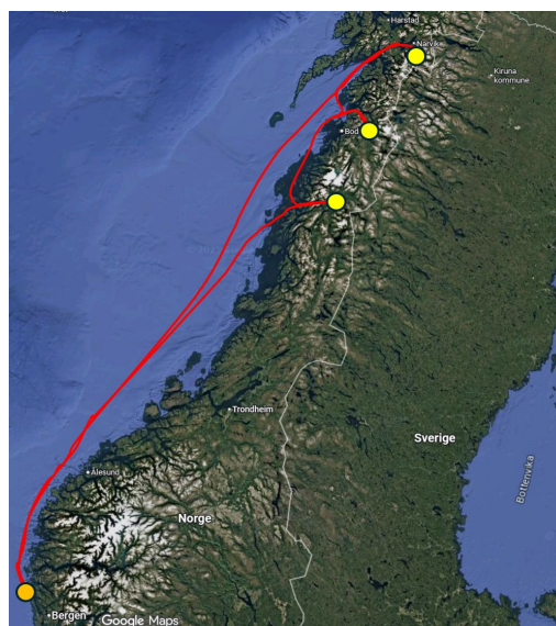
Figure 4-4 The Co-loading sailing route with 3 export terminals (Narvik, Salten and Mo i Rana) and one import terminal at Kollsnes (Northern Lights) [2]
