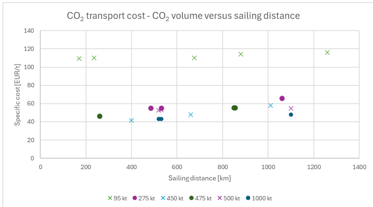
Figure 5-1: Overall CO 2 transport cost trends
