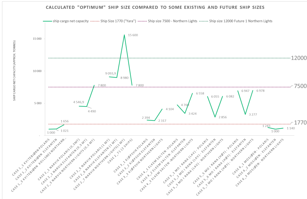
Figure 4-2: Calculated ship sizes for the logistics cases.
