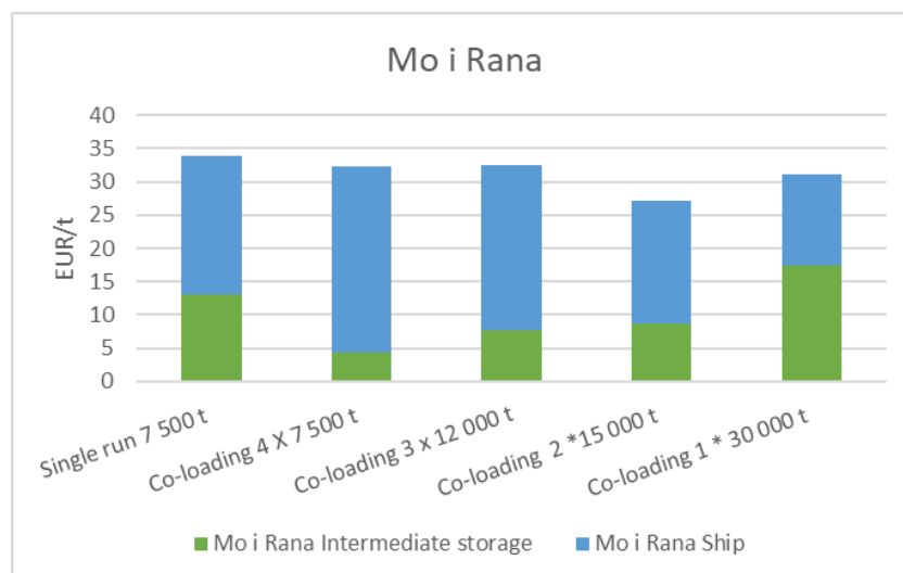
Figure 5-2 Comparison of single run and co-loading for Mo i Rana
