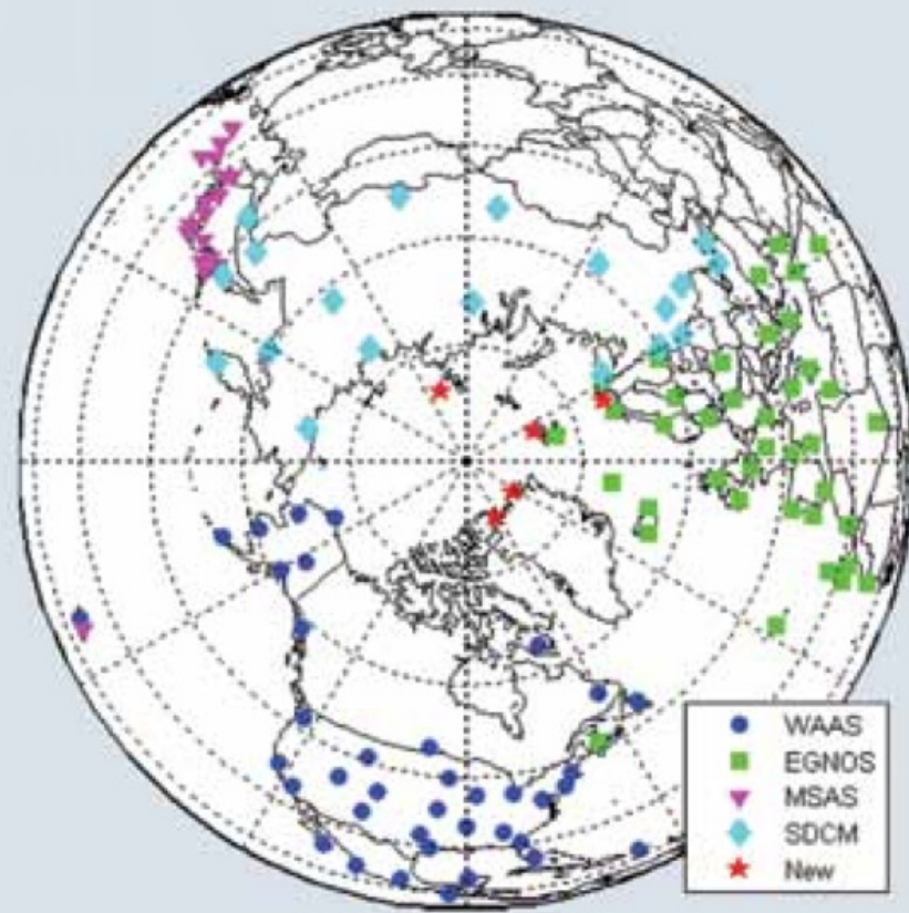
FIGURE 3 Reference stations from WAAS, EGNOS, MSAS, SDCM, and 5 additional stations.
