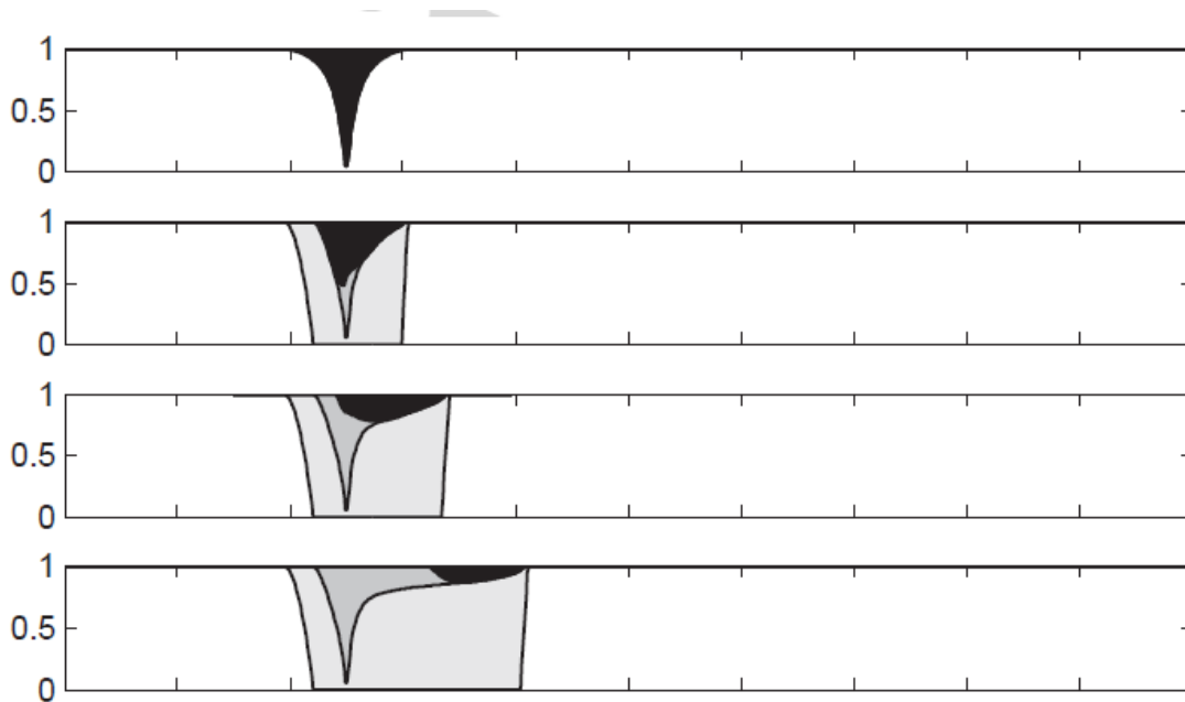
Figure 4: Development of a mobile CO 2 plume (black) under a sloping caprock, where we observe the formation a residually trapped CO 2 (dark grey) and a region of upscaled convective mixing (light gray); Gasda et al. (2011)
