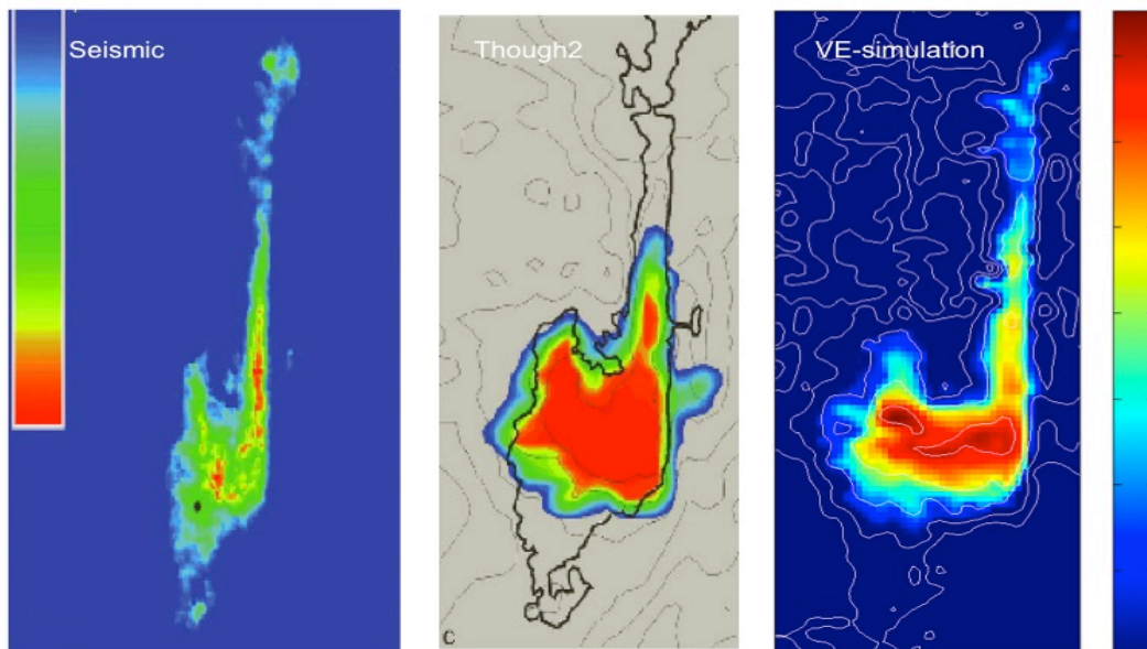
Figure 2: Comparisons of seismic image of CO 2 -plume in the Utsira formation, simulations based on Thought2, and history-matched results based on Vertical Equilibrium simulations. The seismic image and the TOUGH2 simulation are from Chadwick, Noy, Arts, and Eiken, Energy Procedia (2009). 2103-2110. See: http://www.sintef.no/Projectweb/MRST/Gallery/CO2-storage/ for the VE-simulation.
