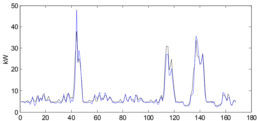
Figure 35. REC of real estate 6 April 2004 (blue curve) compared to the same period in 2001–2003.
