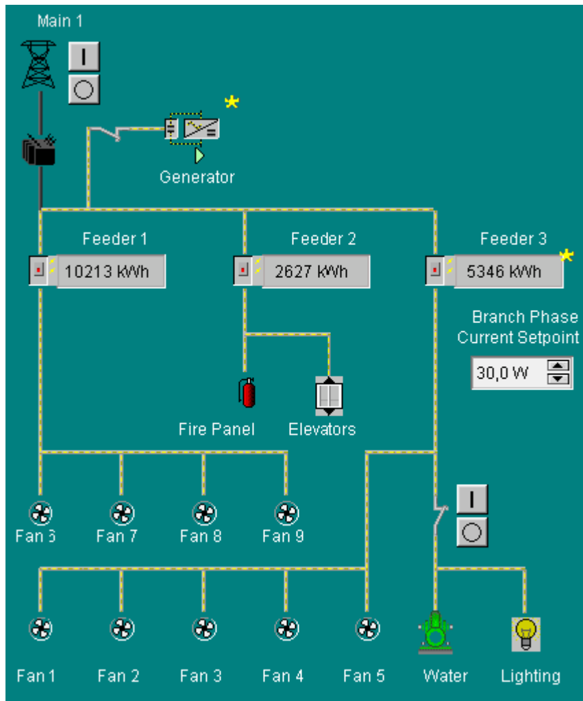
Figure 52. Siemens building automation system controlling loads supplied from different circuits
