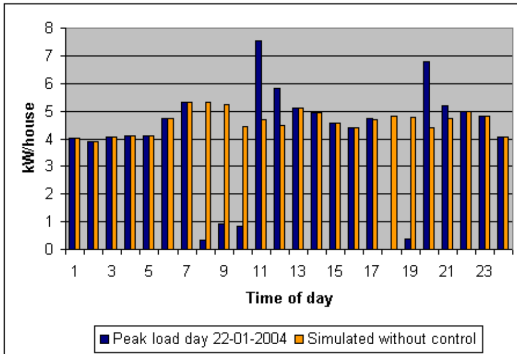
Figure 6. Peak load day 22 January 2004
