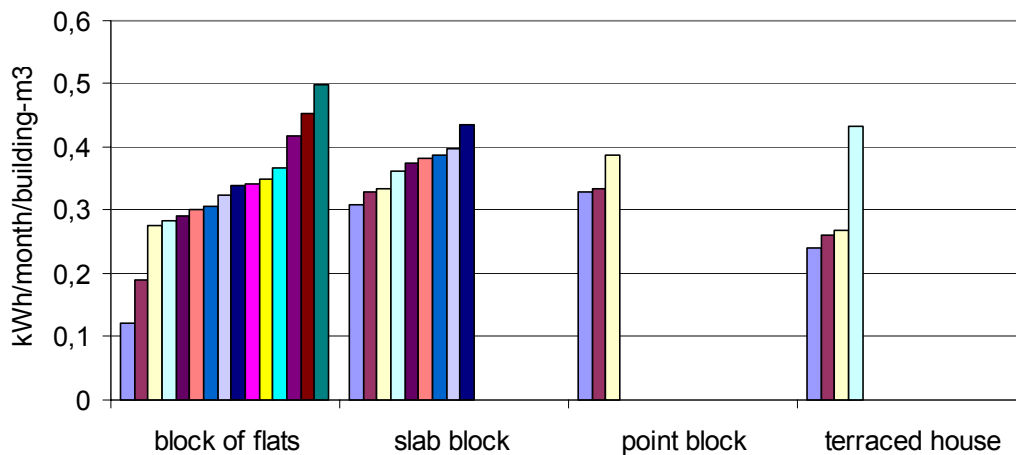
Figure 16. The specific consumption (power / building volume) in different building types in 1994–2002.
