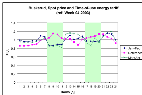
Figure 78. Spot price and ToU Energy tariff
