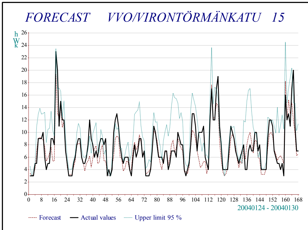
Figure 41. Forecast period 24.1.2004- 30.1.2004. Target is Virontörmätkatu 15 (real estate 29). Confidence interval upper limit added to the figure.
