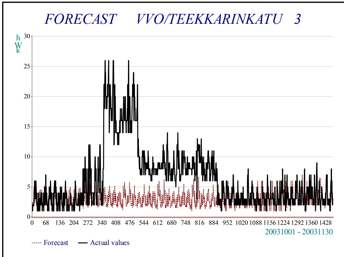
Figure 39. Forecast period 1.10.2003–30.11.2003. Forecasting exceptionally high temporary loads for target real estate 23. On the left, the forecasts slowly starts to follow the exceptionally high loads and results in overoptimistic forecasts for the end of the month. The striking difference between the load and the forecast could be used to set off an automatic alarm email to the property manager. On the right, a target specific calendar is used, where the day span 11.10. – 6.11.2003 is noted as special.
