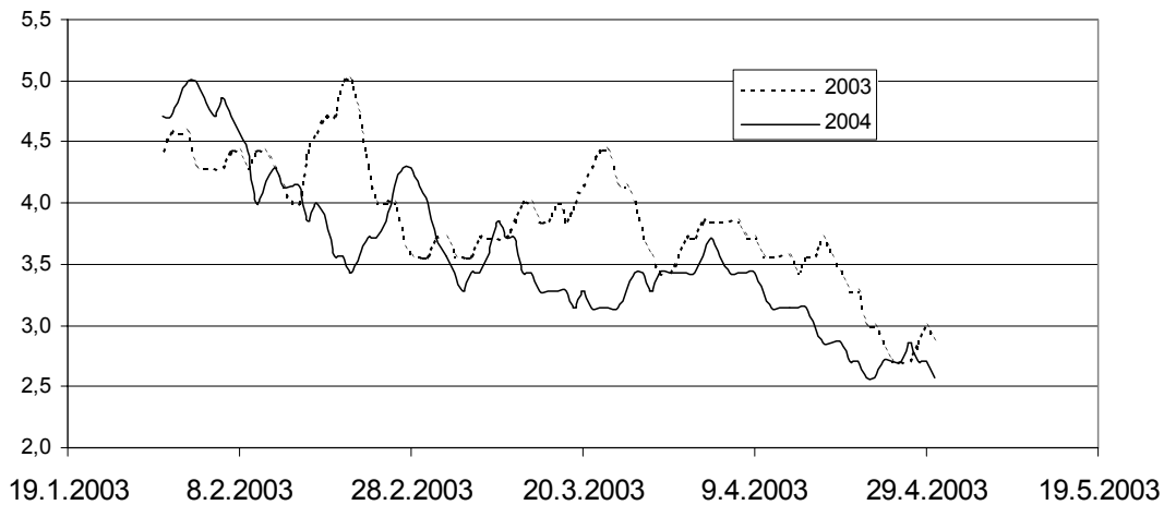
Figure 36. Daily minimum consumption of real estate 6 (kW, 7-day moving average). The dotted line refers to spring 2003 and the solid line to the same days in 2004.
