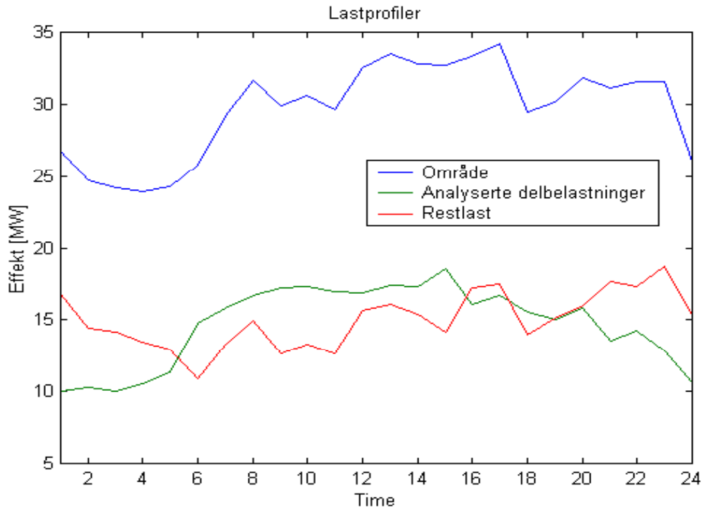
Figure 58. Maximum load profiles for one of the substation (nr 2) supplying the particular customers
