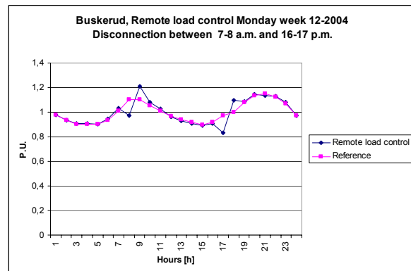
Figure 75. Remote load control
