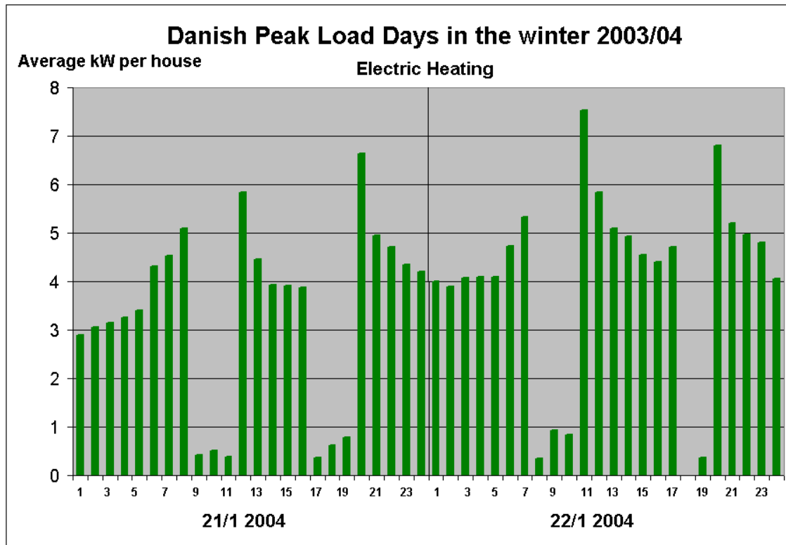
Figure 5. Daily load curves for the two peak load days.
