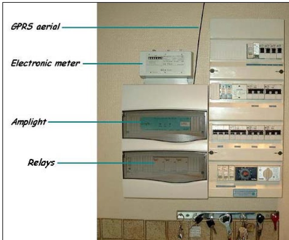
Figure 2. Household installation
