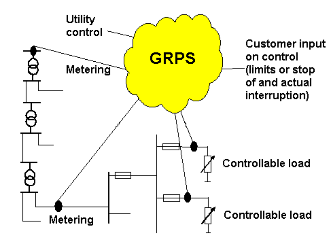
Figure 4. Control by wireless GPRS communication
