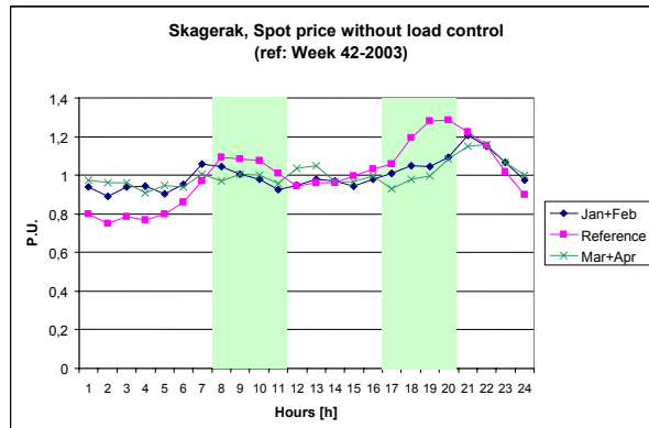
Figure 80. Spot price without load control
