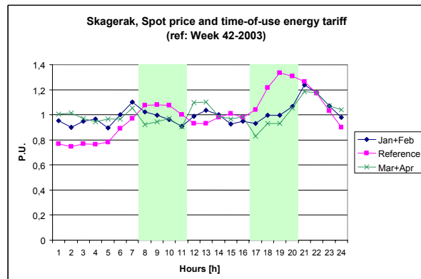
Figure 81. Spot price and ToU Energy tariff
