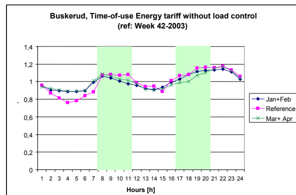
Figure 76. ToU Energy tariff without load control
