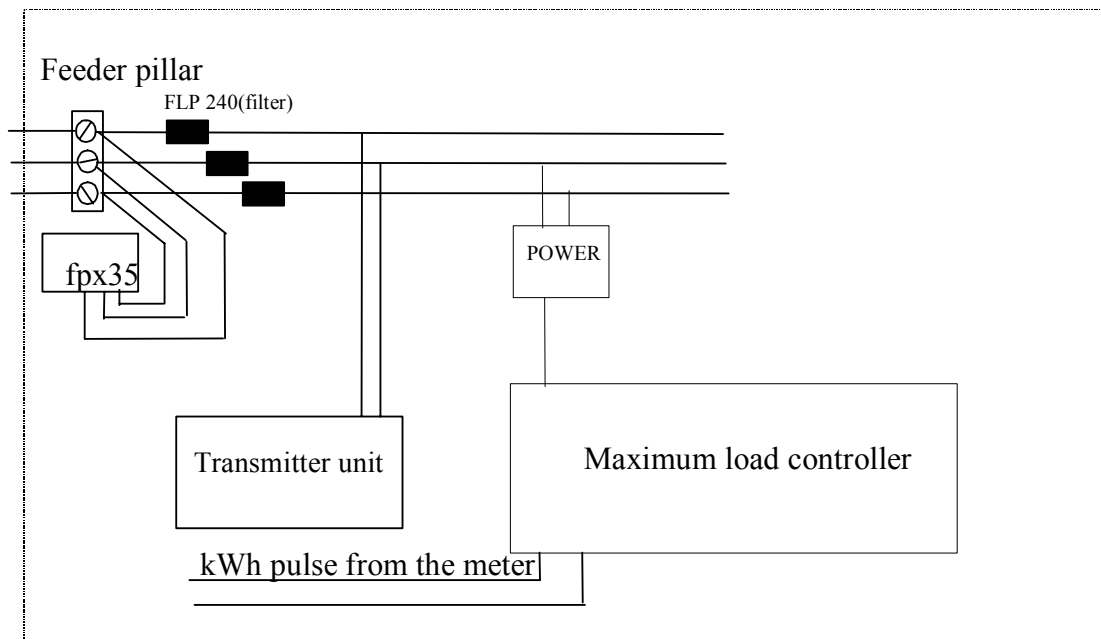
Figure 46. The connection of the maximum load controller in the switchboard room
