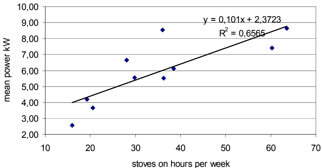
Figure 14. Mean real estate electricity power in 2003 plotted against the total sauna stove-on hours per week. The effect of real estate size has not been subtracted.
