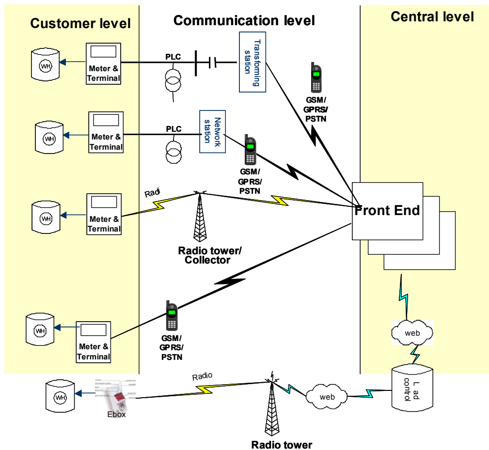
Figure 72. General technology description for the pilot
