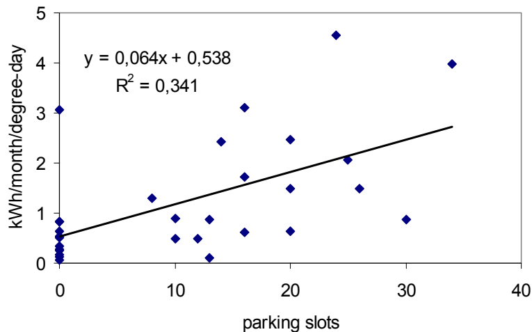
Figure 13. Increase of monthly real estate electricity consumption with heating index number (obtained from data with regression) and the number of heated parking slots.
