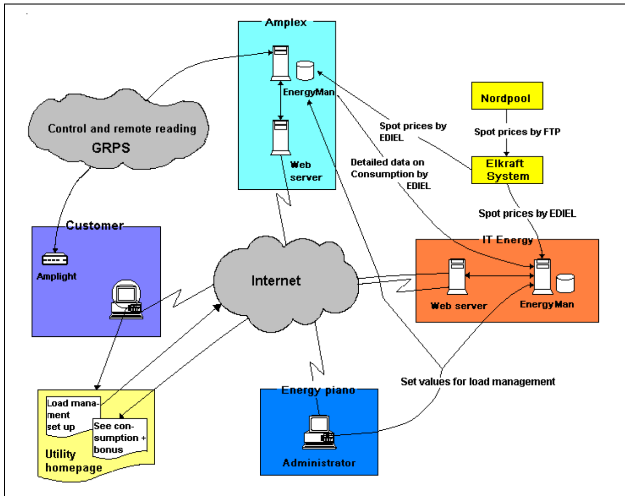
Figure 3. IT configuration in the Danish pilot project
