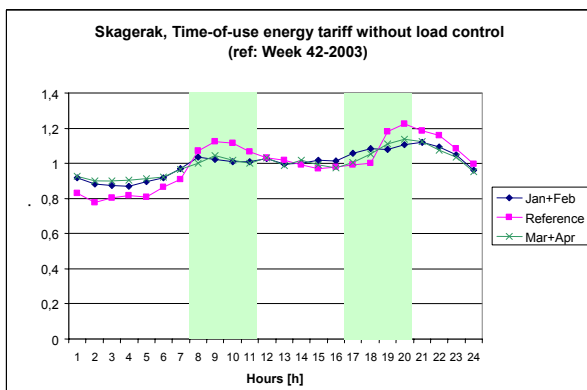
Figure 79. ToU Energy tariff without load control
