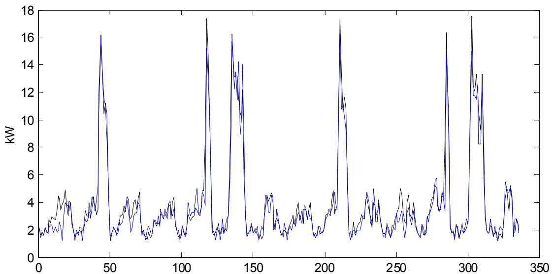
Figure 31. REC of real estate 13 March – April 2004 (blue curve) compared to the same period in 2001–2003. In the figure one month has been averaged into one week and thus two weeks are shown, 168 hours in each.
