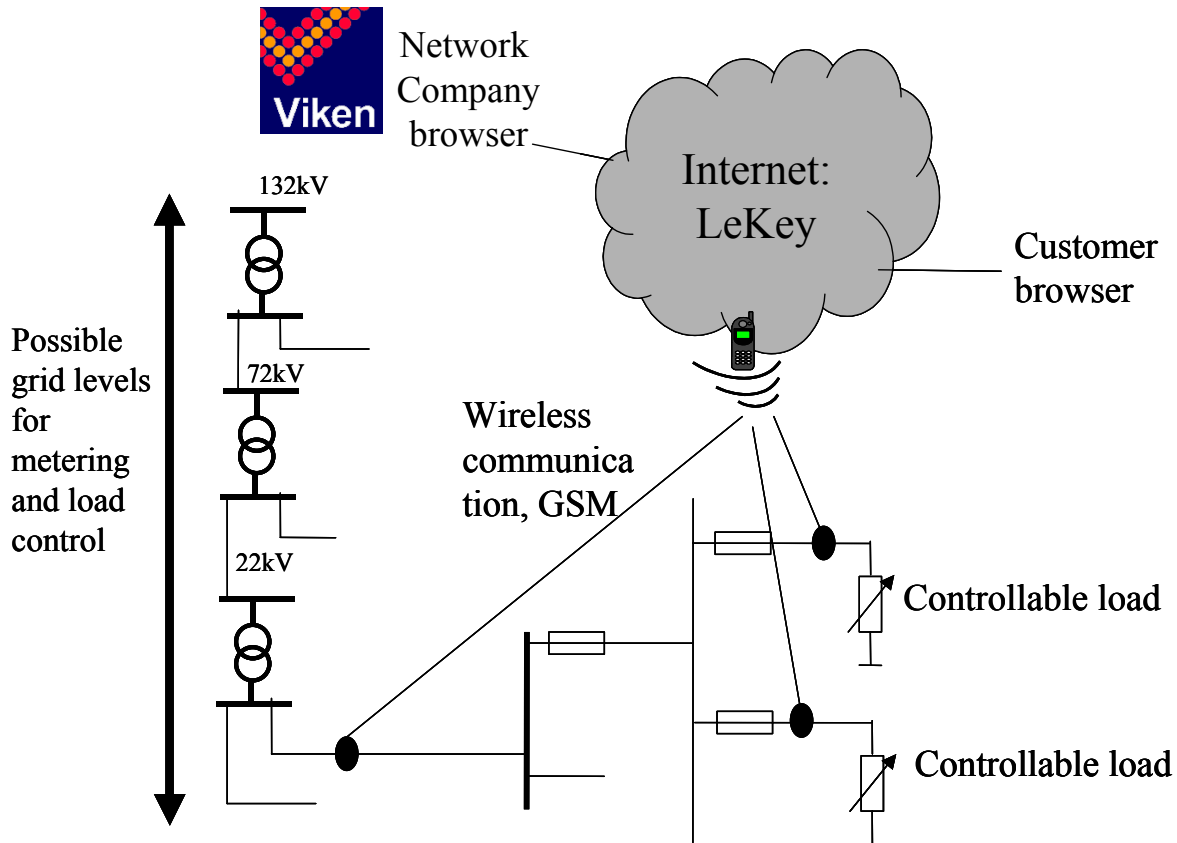
Figure 64. Load control solution of Viken Nett based on Internet and wireless radio communication
