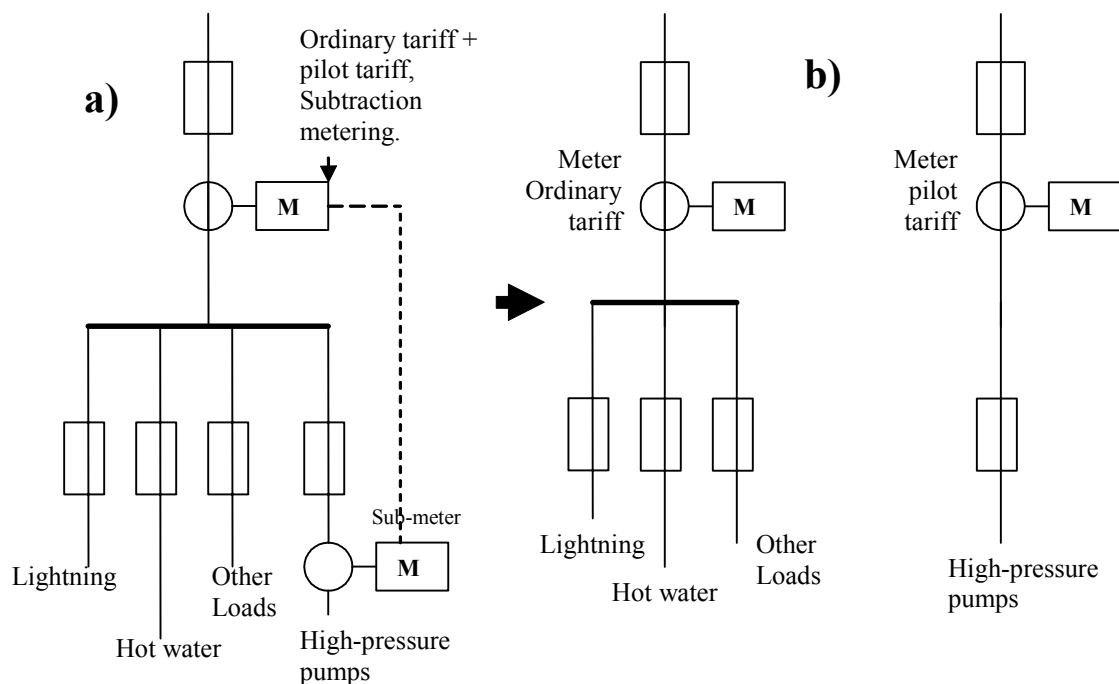
Figure 65. Simplified sketch – metering of controllable and not controllable load
