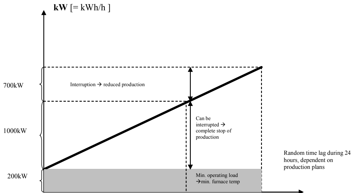
Figure 66. Illustration of possible flexibility of the melting furnaces of the small industry plant
