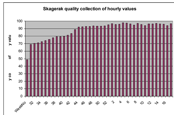
Figure 74. Skagerak Nett, Quality of collection of metered data Aug 2003 – May 2004.
