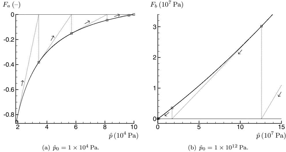
FIG. 1. Convergence for Problem 1 with the initial value lower (left) and higher (right) than the solution. The arrows indicate the direction of successive iterates.
