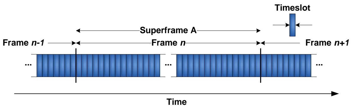
Figure 4: TDMA timeslots, frames and superframes
