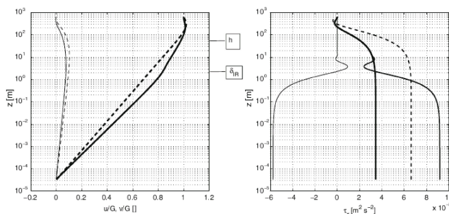
Fig. 1 Left. Wind-speed components. Thick solid line— u -component; thin solid line— v -component; swell is present, \alpha_w = -0.62 ( C_B = -500 , AK = 0.05 ). Thick dashed line— u -component; thin dashed line— v -component, no swell. Right. Stress components (only x -axis components are shown). Thick solid line—total stress; medium solid—turbulent stress; thin solid—wave-induced stress, swell is present. Dashed line—turbulent stress, no swell. The heights of the inner region \delta_{JR} and the atmospheric surface layer h are shown by horizontal lines crossing the vertical axis
