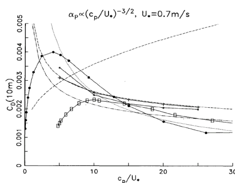
FIG. 16. Drag coefficient for z = 10 m with Phillips parameter \alpha_p = 0.57(c_p/U_*)^{-3/2} and friction velocity U_* = 0.7 m s ^{-1} . Solid lines: Model results. With solid circles, present model; with asterisks, Janssen (1989); with plus signs, Jenkins (1992); with rectangles, Nordeng (1991); dotted line: curve fitted by Geernaert et al. (1987) to field experimental results with a range of values of U_* ; close dashed line (long dashes): from the relation of Toba and colleagues [Toba and Koga 1986, Eqs. (9) and (10)]; dash-dotted line: from HEXMAX measurements (Maat et al. 1991); dash-and-three-dots line: from Lake Ontario measurements (Donelan 1990).
