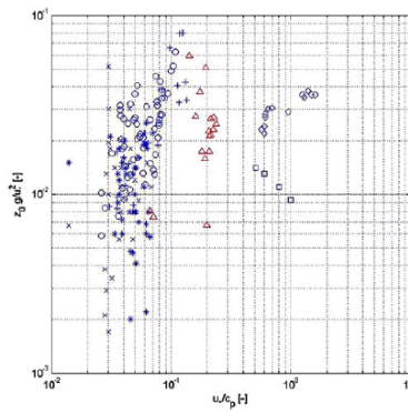
Figure 14. Charnock parameter z_0g/u^2 versus inverse wave age u/c_p . Symbols indicate data. Circles: HEXMAX [Janssen, 1997]; pluses: Lake Ontario; stars: Atlantic Ocean, long fetch; x-marks: Atlantic Ocean, limited fetch [Donelan et al., 1993]; diamonds: wave tank [Keller et al., 1992]. Data are compiled from Donelan et al. [1993], their Figure 2. Triangles: present paper.
