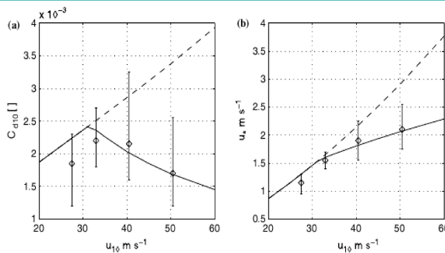
Figure 1. (a) Drag coefficient versus the wind speed, (b) Friction velocity versus the wind speed. Solid line, according to the resistance law (11); dashed line, according to the Charnock relation (3); open circles, data by Powell et al. (2003).
