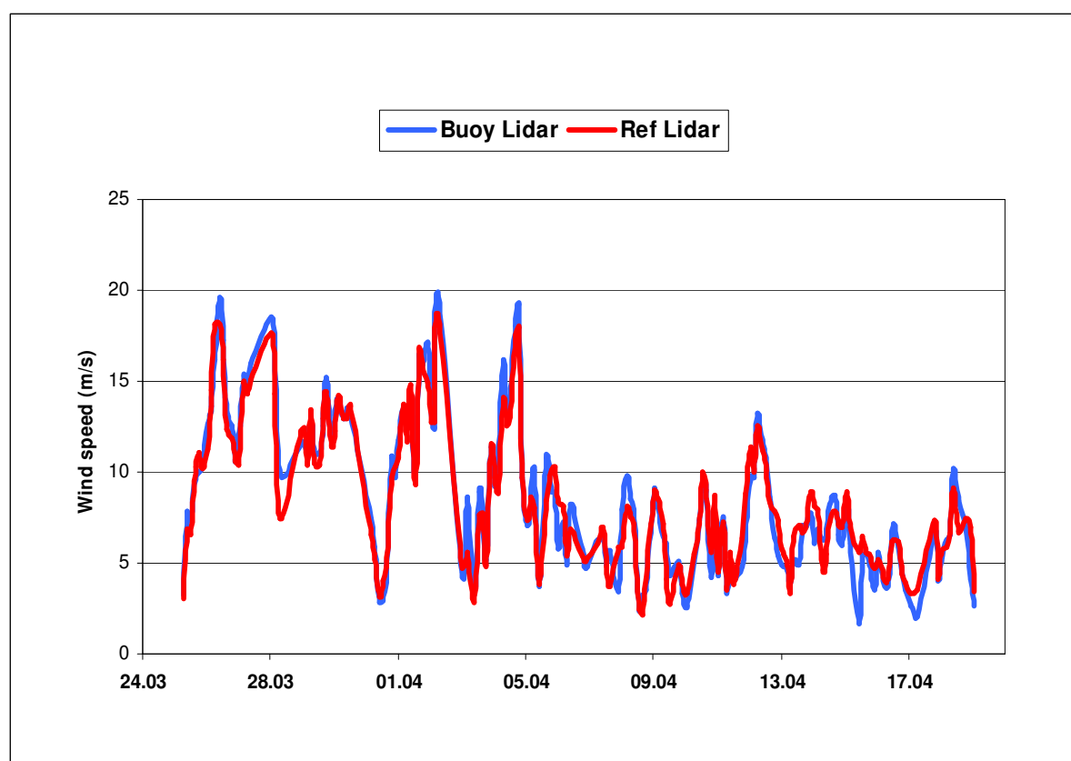
Field test Titran – Wind speed at 53m
